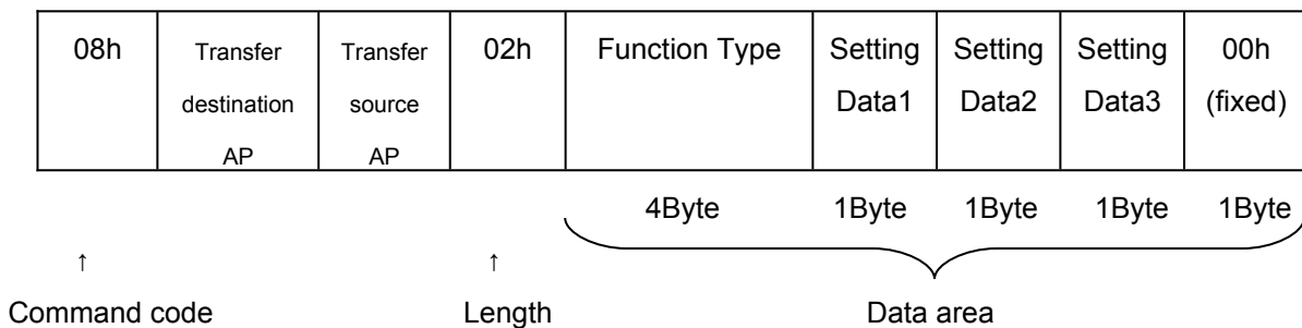
Fig. 6-7 Data Transfer Frame Composition During [End Adjustment]
